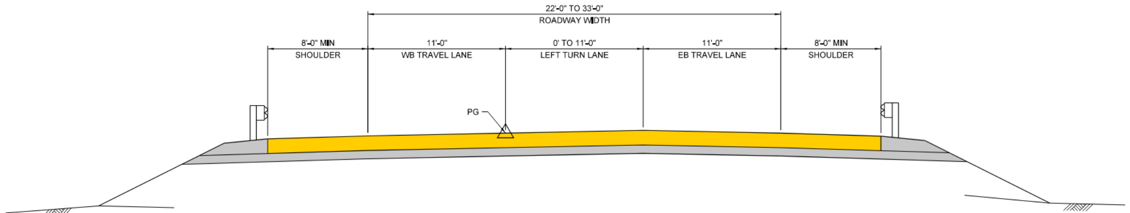
PA 663 TYPICAL SECTION
