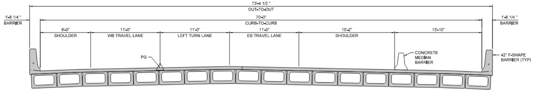
PA 663 OVER UNAMI CREEK
