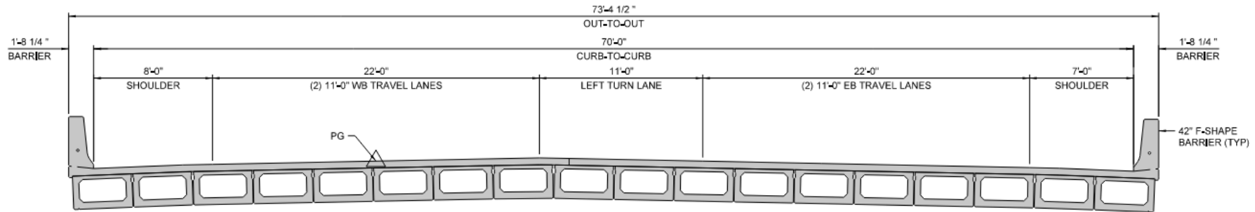
PA 663 OVER UNAMI CREEK (FUTURE)
