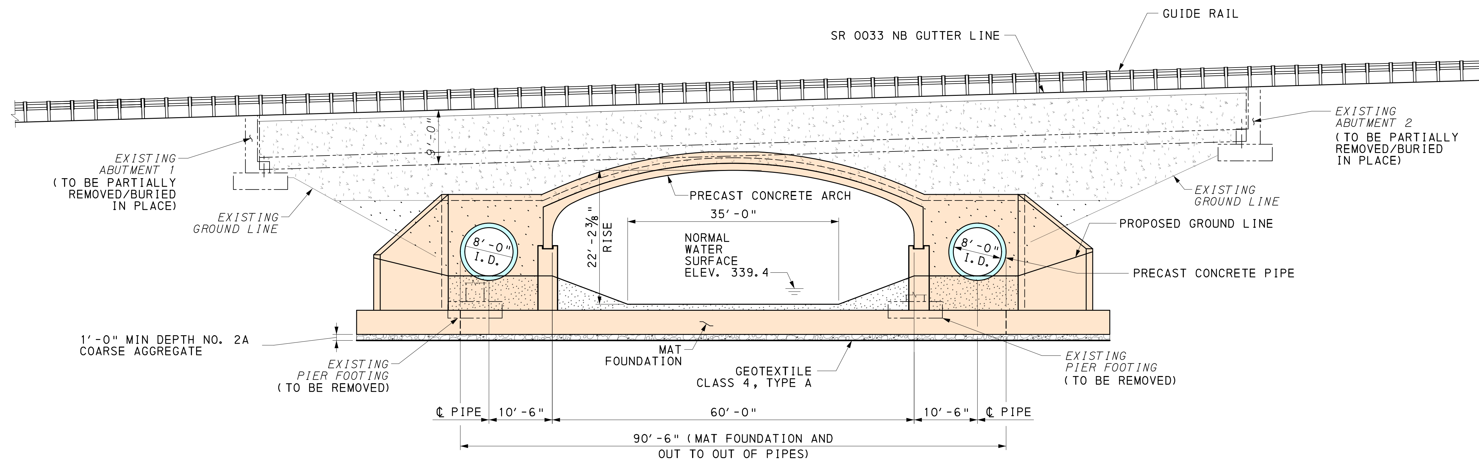
OUTLET STRUCTURE ELEVATION
