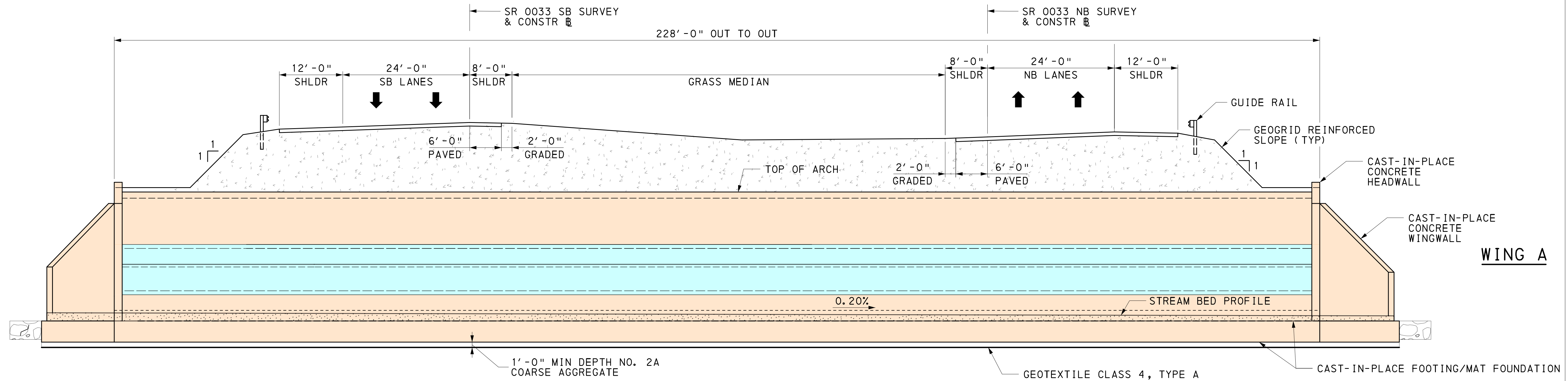
TYPICAL STRUCTURE SECTION
