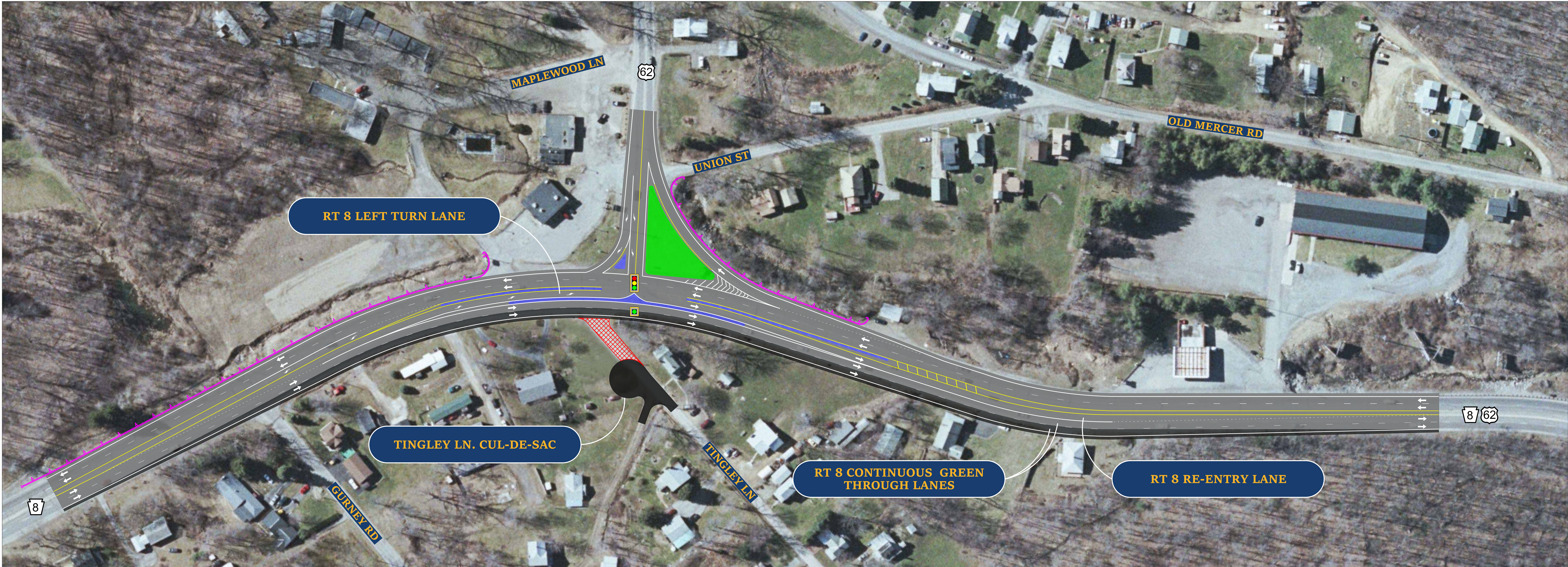
ALT 4C - Left-Turn Acceleration (LTA) / 2-Lane (Curbed / Signalized)
