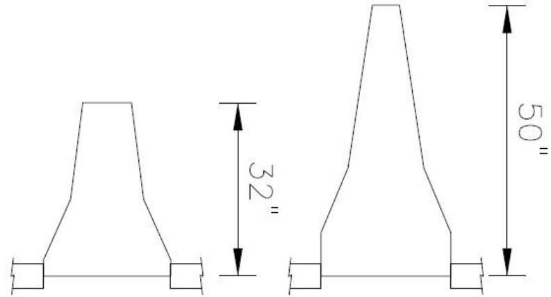
EXISTING CONCRETE MEDIAN BARRIER
